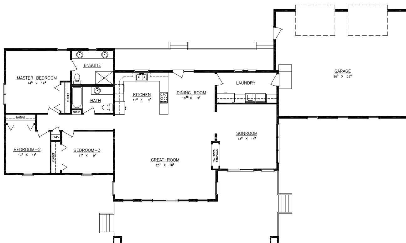
FLOOR PLAN
